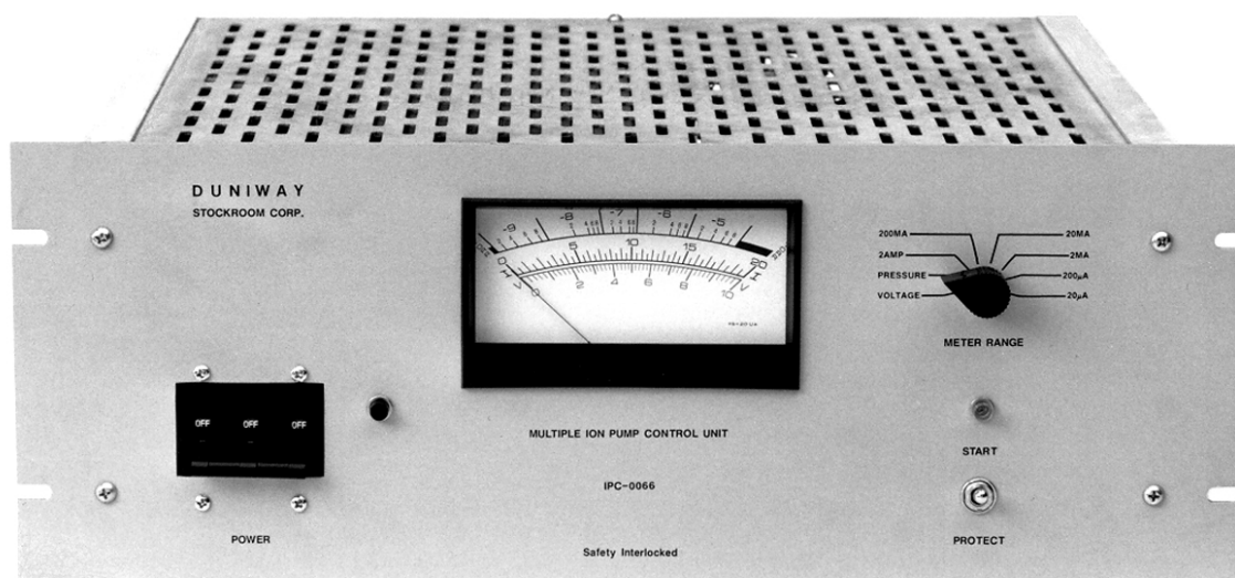
Figure 7: Front Panel
